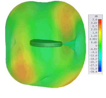
Element 2: Typical 3D Pattern (5.4GHz)
