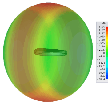
Element 1: Typical 3D Pattern (2100MHz)
